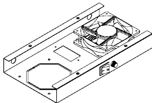
PERSPECTIVE VIEW
