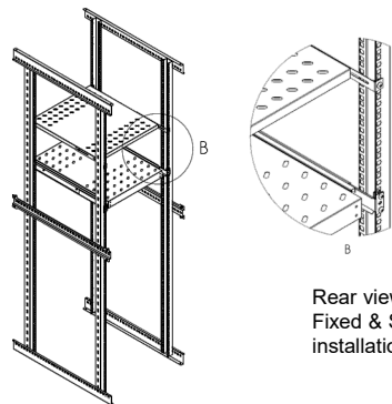
Front view Fixed & Sliding shelf installation
